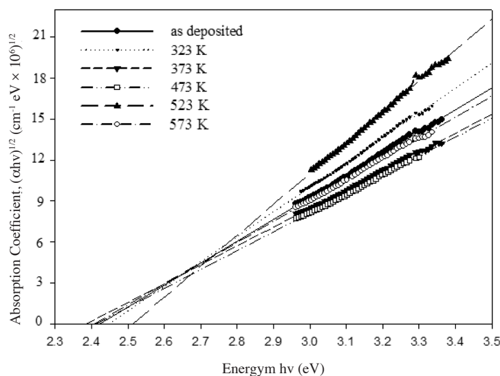
FIGURE 3. Plot of (\alpha hv)^{1/2} against hv
